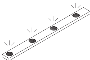
DA-LED Elemento LED a terra luce wall-wash LED floor light wall-wash L. 56 x P. 3 x H. 2 cm
